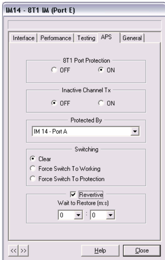
Figure 6: Octal T1 IM Configuration Dialog APS Tab
