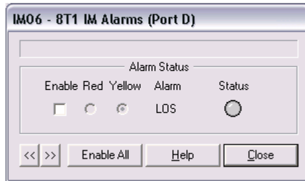
Figure 8: Octal T1 IM Alarm Monitor Setup Window
