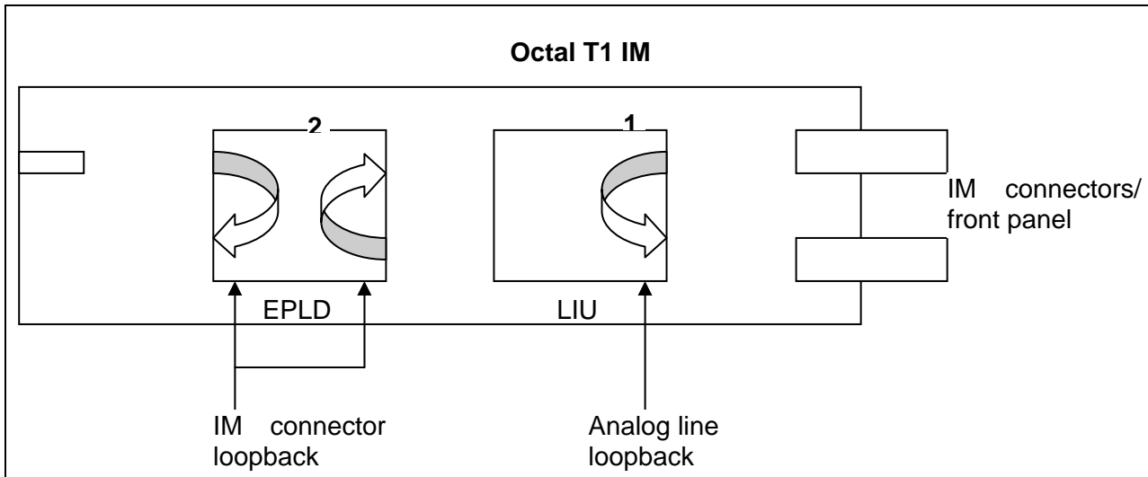
Figure 7: Octal T1 IM loop-back options
